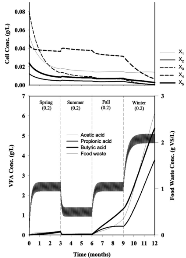
Fig. 8. Model prediction of solid food waste consumption, VFA, and bacterial group concentrations using a repeated input of 0.2 g VS L -1 day -1 , without temperature control.
