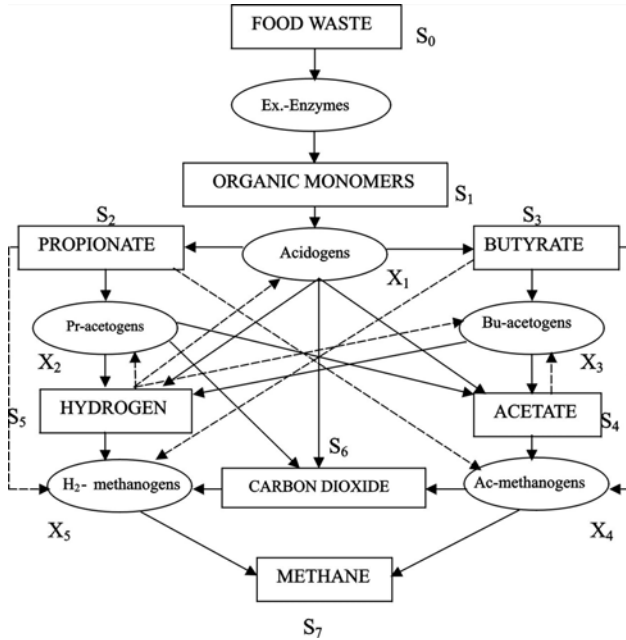
Fig. 2. Outline of the model ( —material flow, -inhibition). organic monomers (S 1 ) and their-degrading acidogens (X 1 ), propionate (S 2 ) and its-degrading acidogens (X 2 ), butyrate(S 3 ) and its degrading acidogens (X 3 ), acetic acids (S 4 ) and acetoclastic methanogens (X 4 ), hydrogen (S 5 ) and hydrogenotrophic methanogens (X 5 ).Carbon dioxide (S 6 ) and Methane (S 7 ). Sample explanation: organic monomers (S 1 ) are decomposed by acetogens groups (X 1 ) into S 4 , S 2 , S 3 , S 5 and S 6 . These reactions are inhibited by hydrogen, S 5 .
