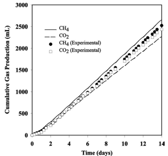
Fig. 6. Model prediction versus observed values of cumulative gas production in a repeated input operation at 2 g VS L -1 day -1 (Temperature = 35°C).
